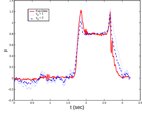
(a) Braking #1
