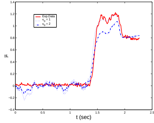
(b) Braking #2
