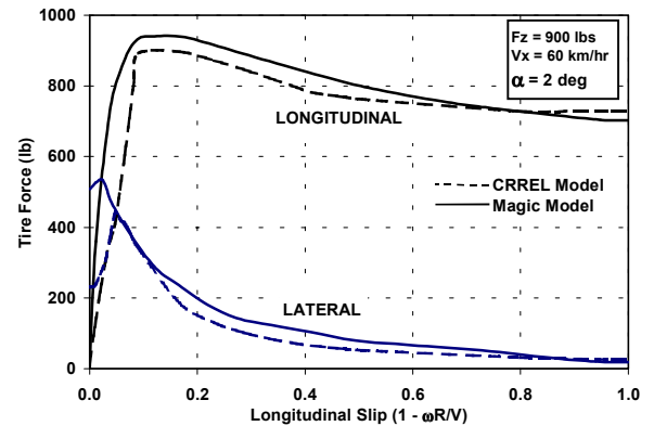
Figure 9: Tire Forces on Dry Pavement - \alpha = 2 \text{ deg}
