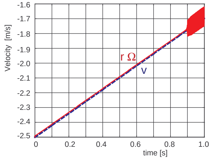
Figure 4 – Results of the explicit Euler algorithm
