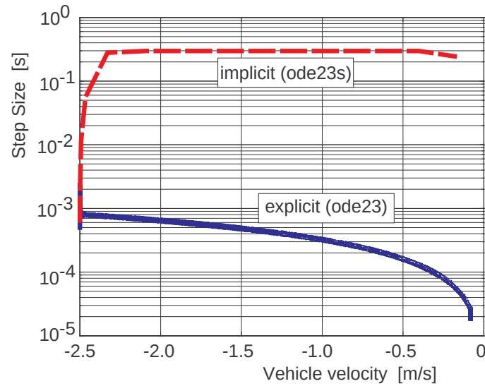
Figure 5 – Step sizes for explicit and implicit solver
